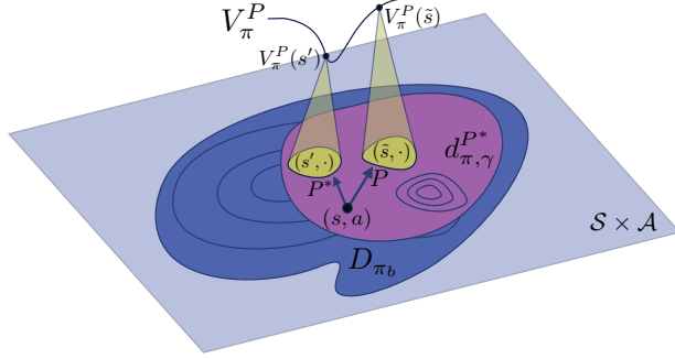
Figure 1: A visual representation of the model-based OPE objective in Eq. (10). The error at every point (s, a) in D_{\pi_b} is the difference between V_{\pi}^P(\tilde{s}) (induced by following P ) and V_{\pi}^P(s') (induced by following P^* ). We weight the over/under-counting of some points (s, a) in D_{\pi_b} to make it look like the data was actually generated by d_{\pi, \gamma}^{P^*} . Summing up all the errors exactly yields the OPE error of using P as a simulator.
